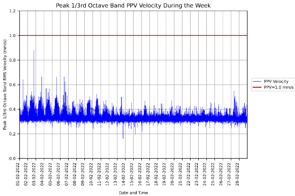
Figure 2: Measured vibration levels for 01/02/2022 to 28/02/2022 at the KR - Animal House.
