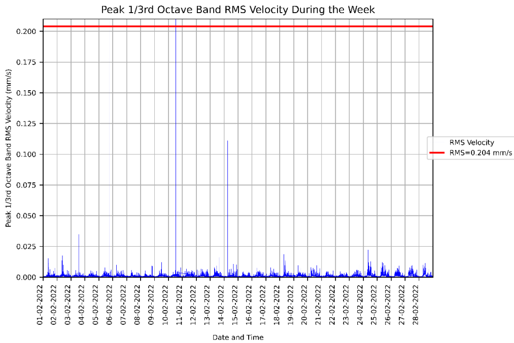
Figure 3: Measured RMSV vibration levels for 01/02/2022 to 28/02/2022 at the CH - Mental Health Utility - Wade Ward.
