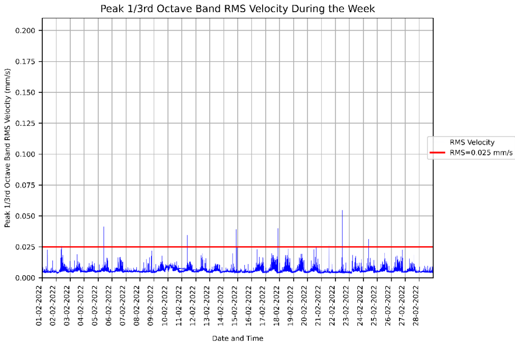
Figure 3: Measured RMSV vibration levels for 01/02/2022 to 28/02/2022 at the KR - L4 Lab 9.
