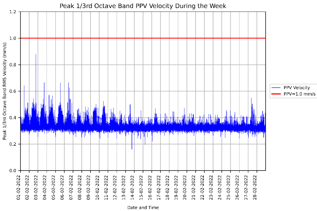
Figure 5: Measured PPV vibration levels for 01/02/2022 to 28/02/2022 at the KR - Animal House.
