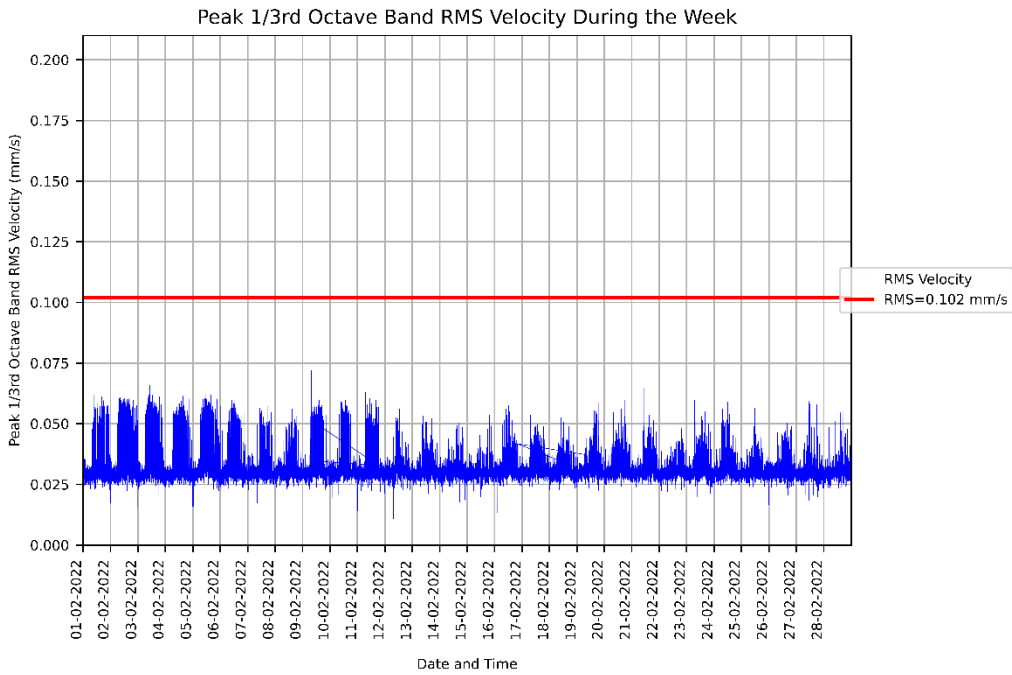
Figure 4: Measured RMSV vibration levels for 01/02/2022 to 28/02/2022 at the KR - Animal House.
