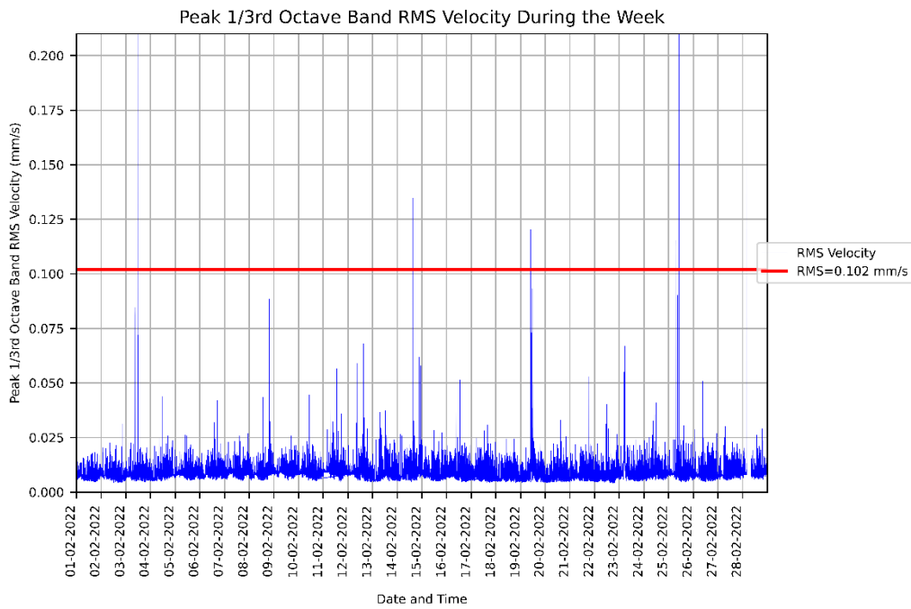
Figure 3: Measured RMSV vibration levels for 01/02/2022 to 28/02/2022 at the CASB level 3 Surgical Suite.
