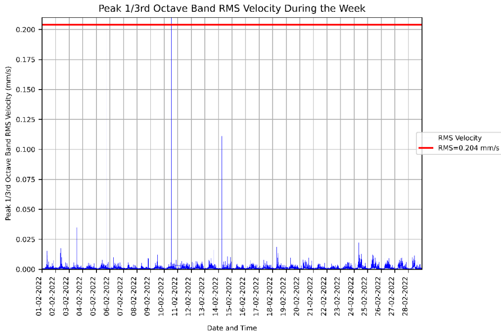
Figure 1: Measured RMSV vibration levels for 01/02/2022 to 28/02/2022 at the CH - Mental Health Utility - Wade Ward.
