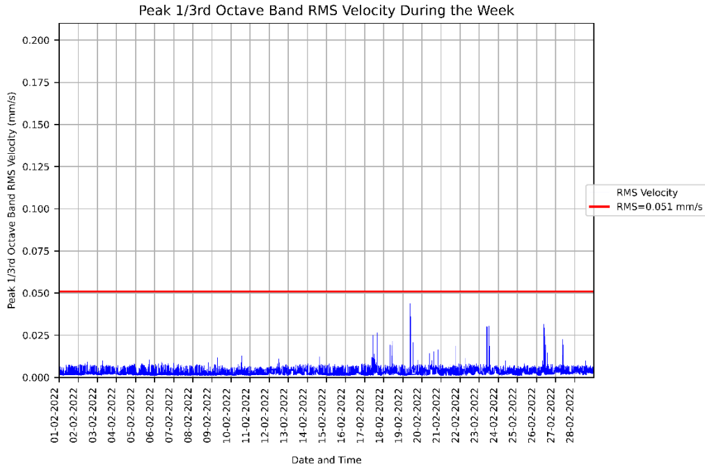
Figure 3: Measured RMSV vibration levels for 01/02/2022 to 28/02/2022 at the CASB Level 2 MRI.
