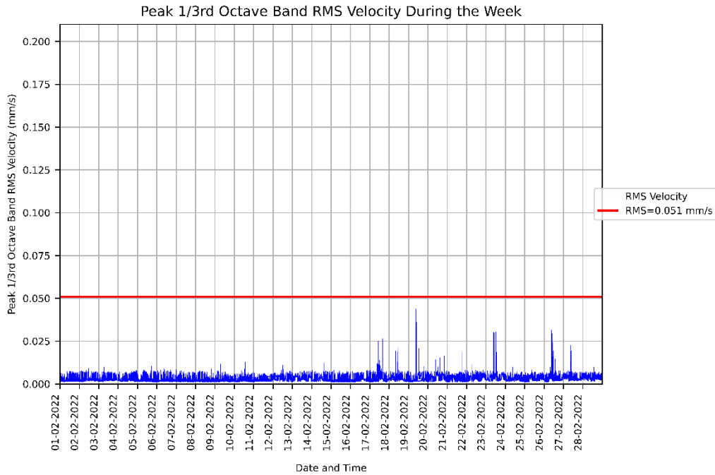
Figure 1: Measured RMSV vibration levels for 01/02/2022 to 28/02/2022 at the CASB Level 2 MRI.
