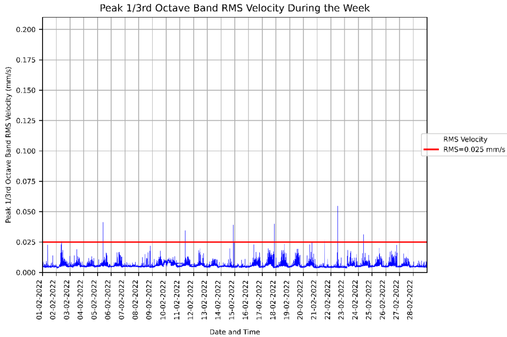
Figure 1: Measured RMSV vibration levels for 01/02/2022 to 28/02/2022 at the KR - L4 Lab 9.
