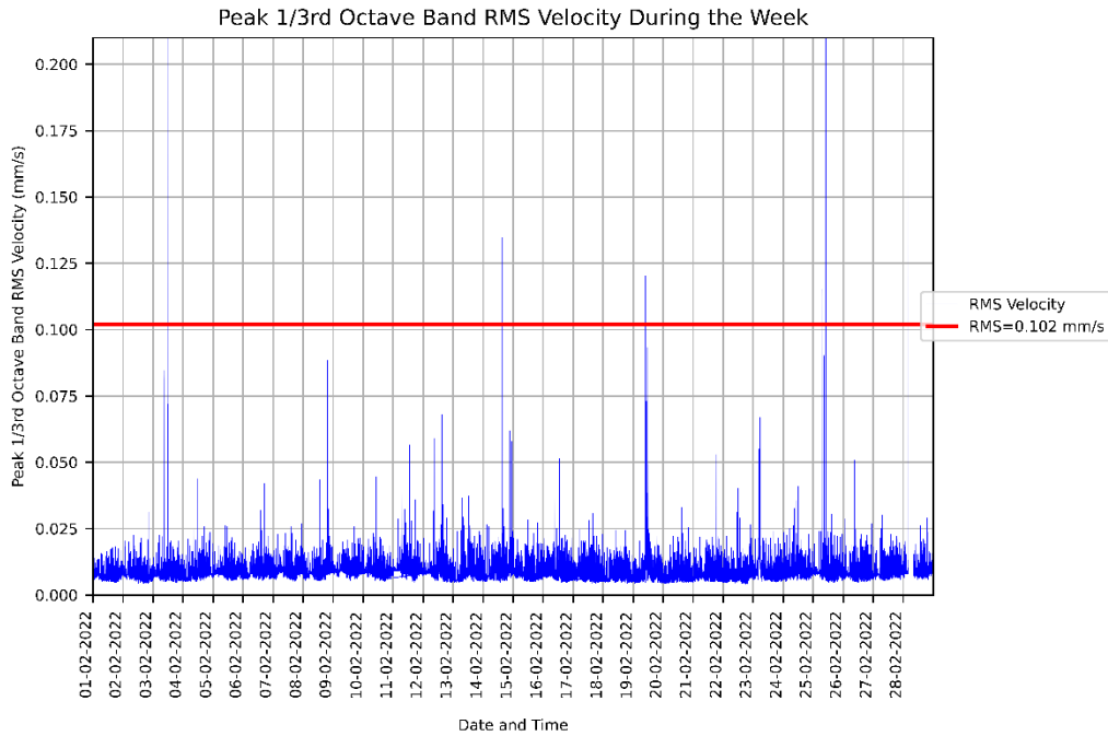
Figure 1: Measured RMSV vibration levels for 01/02/2022 to 28/02/2022 at the CASB level 3 Surgical Suite.
