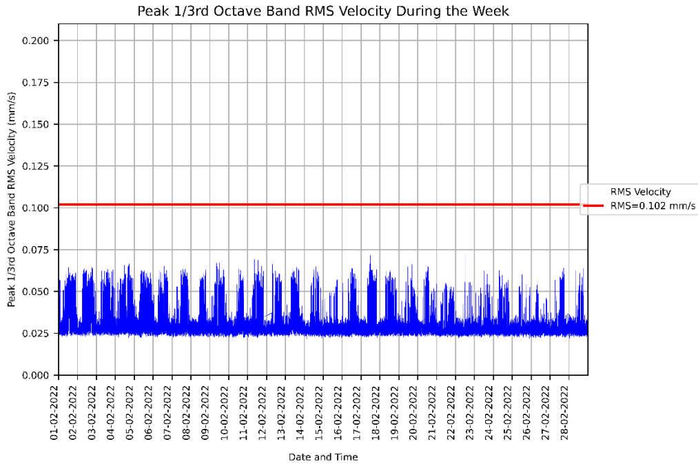
Figure 1: Measured RMSV vibration levels for 01/02/2022 to 28/02/2022 at the CHW - L1 Lab.
