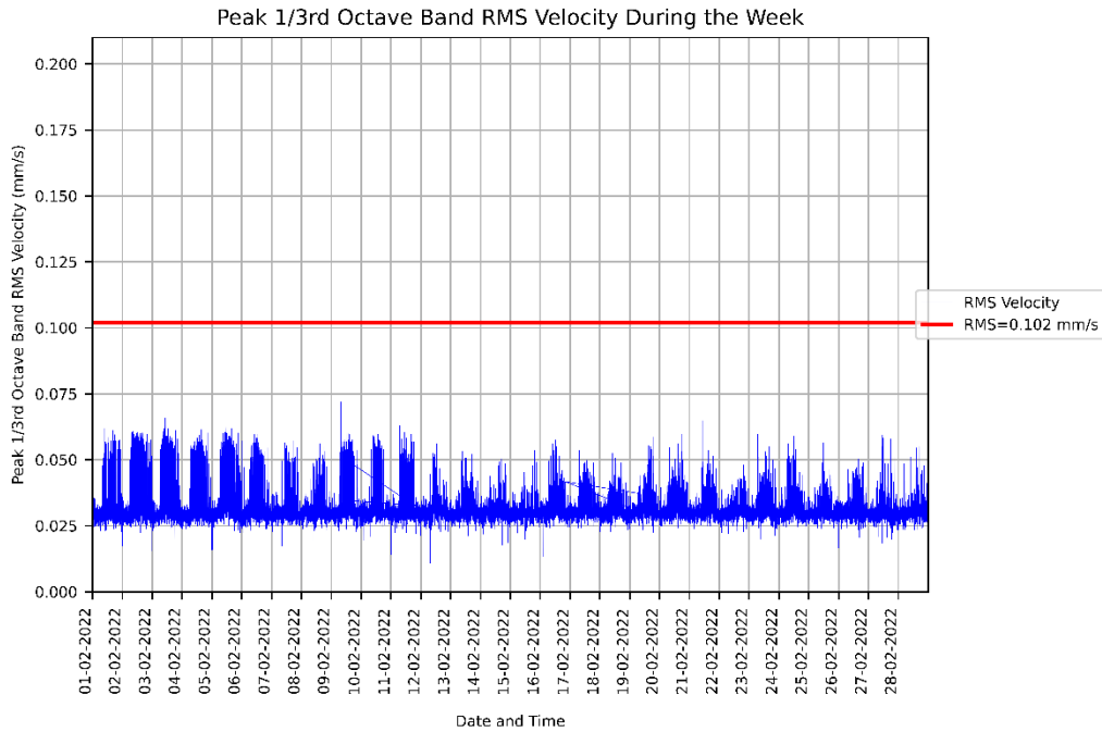
Figure 1: Measured RMSV vibration levels for 01/02/2022 to 28/02/2022 at the KR - Animal House.
