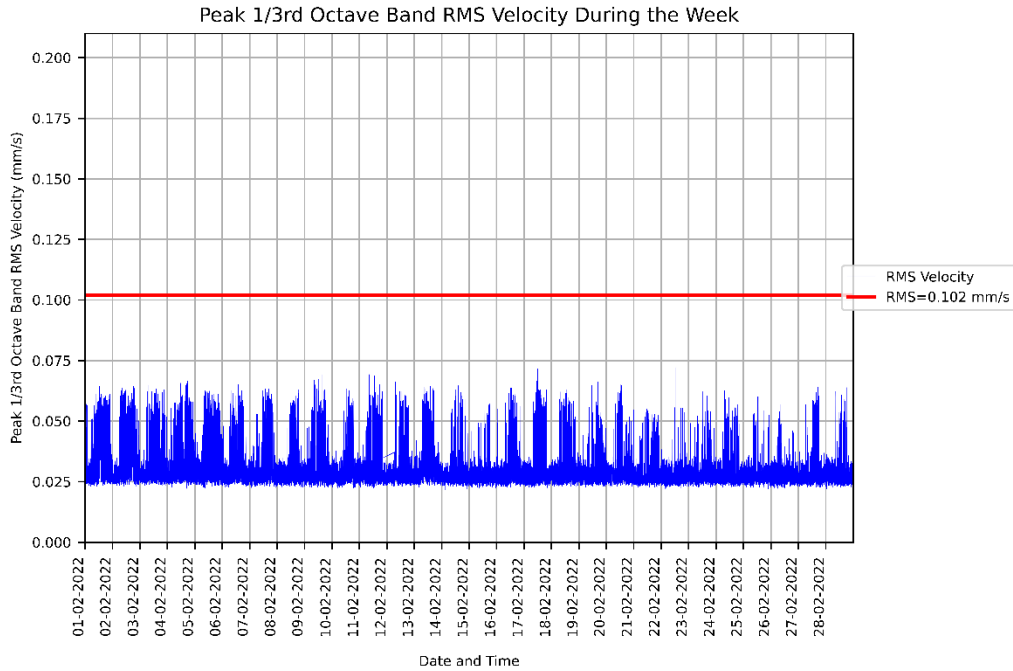
Figure 3: Measured RMSV vibration levels for 01/02/2022 to 28/02/2022 at the CHW - L1 Lab.
