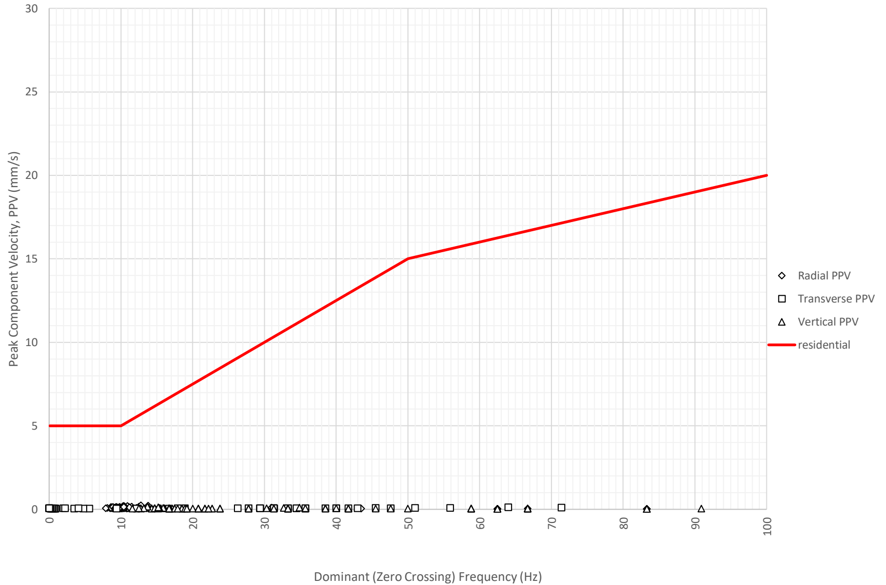
Frequency Content of Vibration Levels at Nepean Hospital Stage 2 - Tresillian Building (ETM7426) on 18-01-2024
