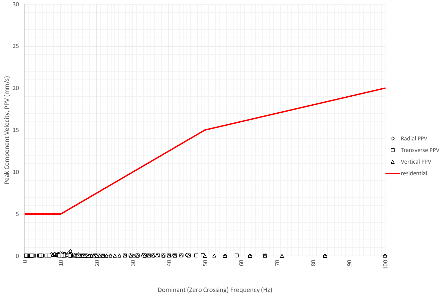
Frequency Content of Vibration Levels at Nepean Hospital Stage 2 - Tresillian Building (ETM7426) on 24-01-2024
