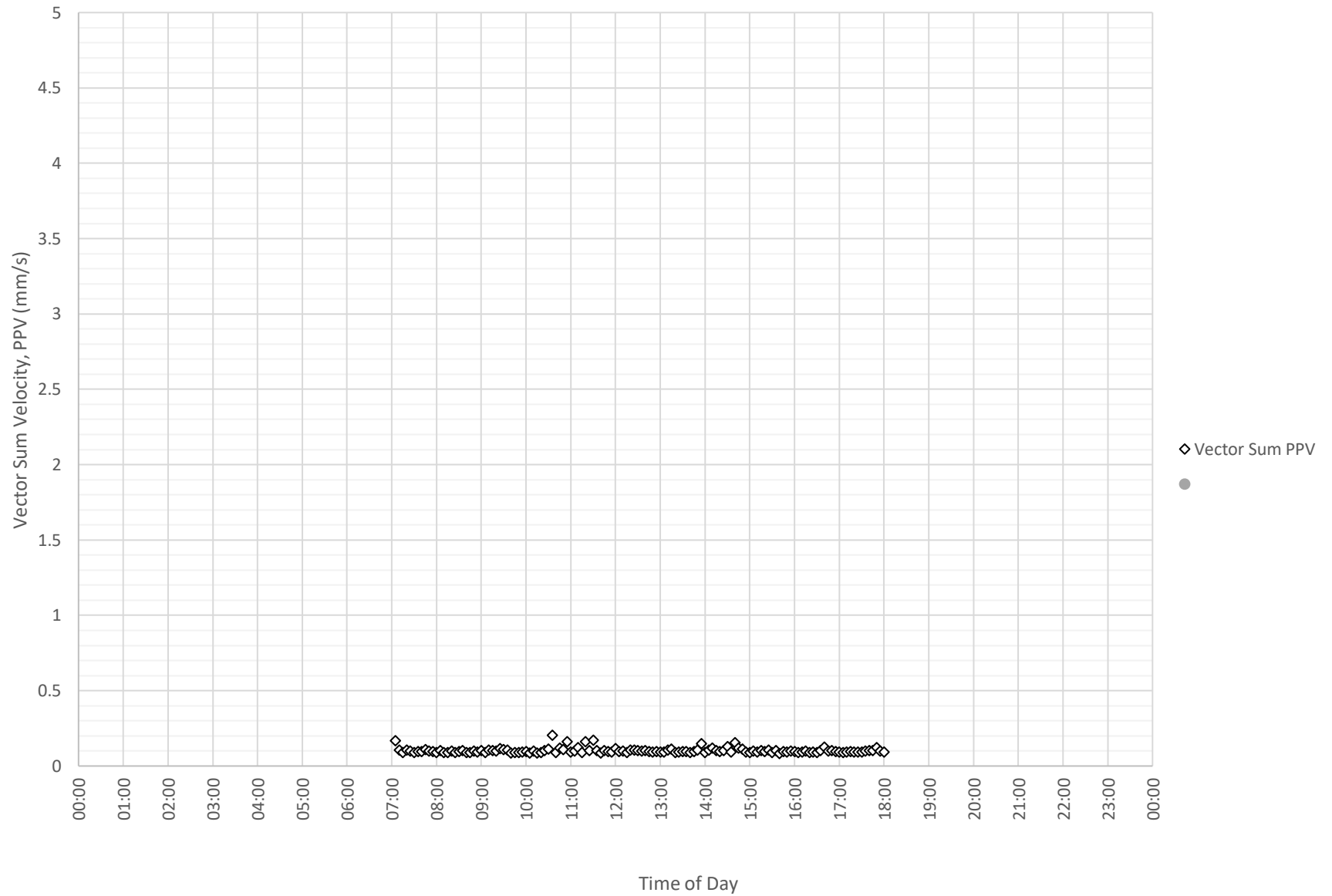
Daily Monitored Vibration Levels at Nepean Hospital Stage 2 - Level 2 Waiting Area (ETM7381) on 15-01-2024
