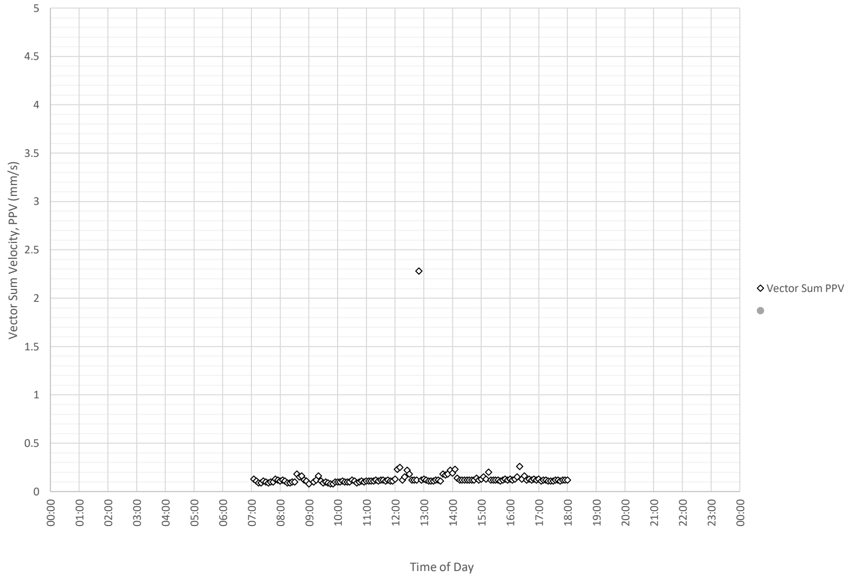
Daily Monitored Vibration Levels at Nepean Hospital Stage 2 - TB1 Corridor (ETM7280) on 23-01-2024
