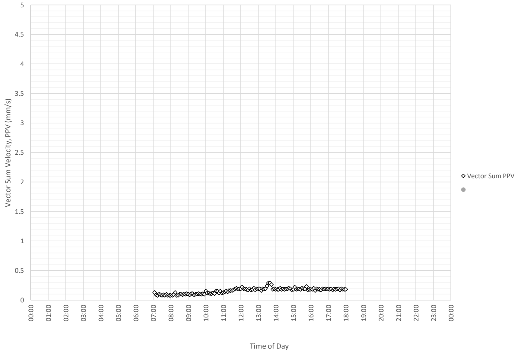
Daily Monitored Vibration Levels at Nepean Hospital Stage 2 - TB1 Corridor (ETM7280) on 24-01-2024
