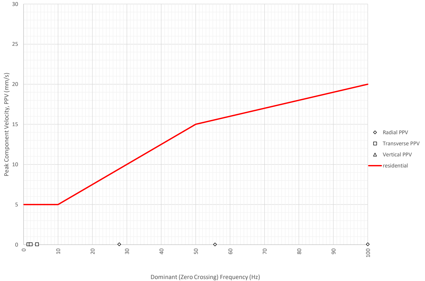
Frequency Content of Vibration Levels at Nepean Hospital Stage 2 - Tresillian Building (ETM7426) on 21-01-2024
