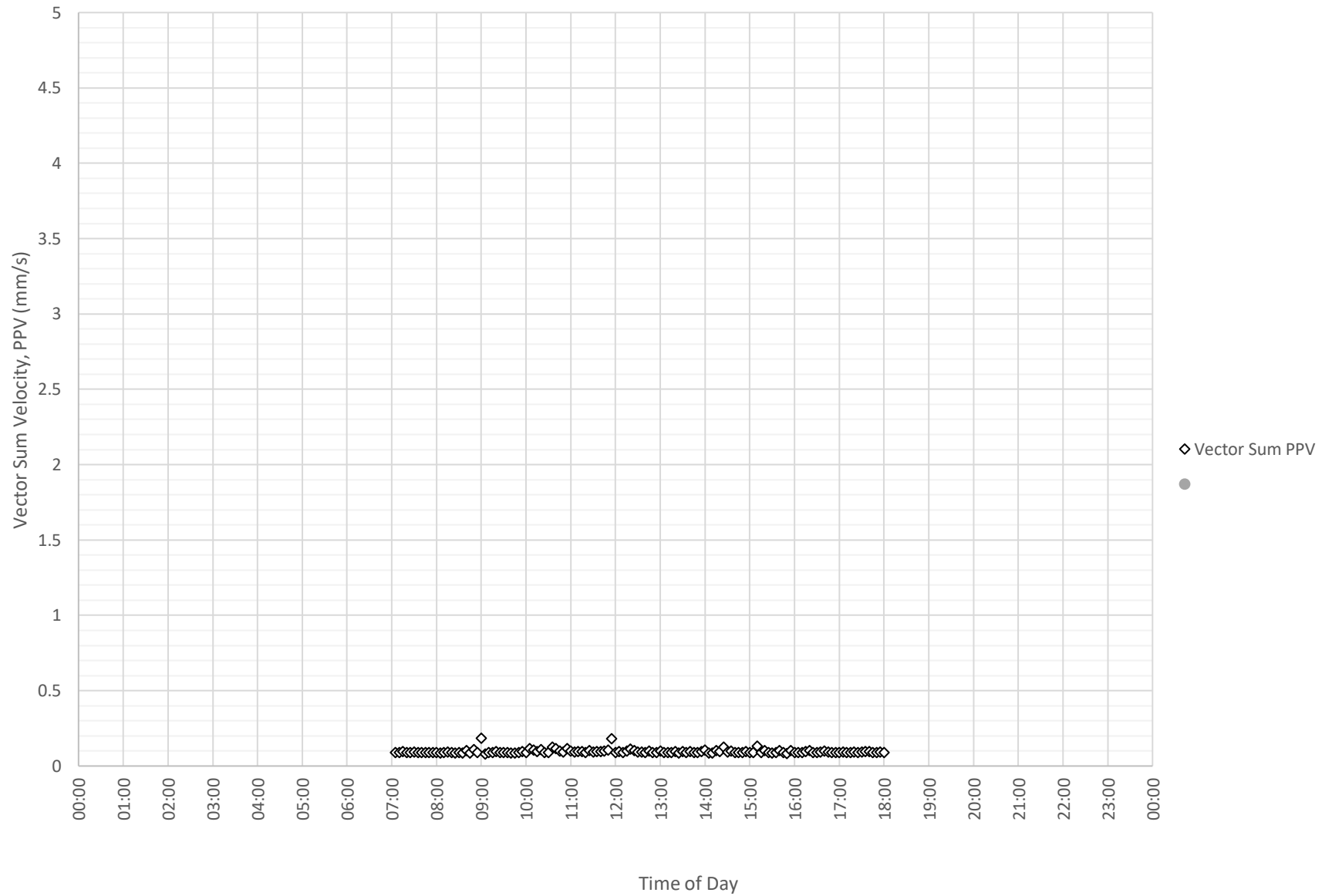
Daily Monitored Vibration Levels at Nepean Hospital Stage 2 - Level 2 Waiting Area (ETM7381) on 20-01-2024
