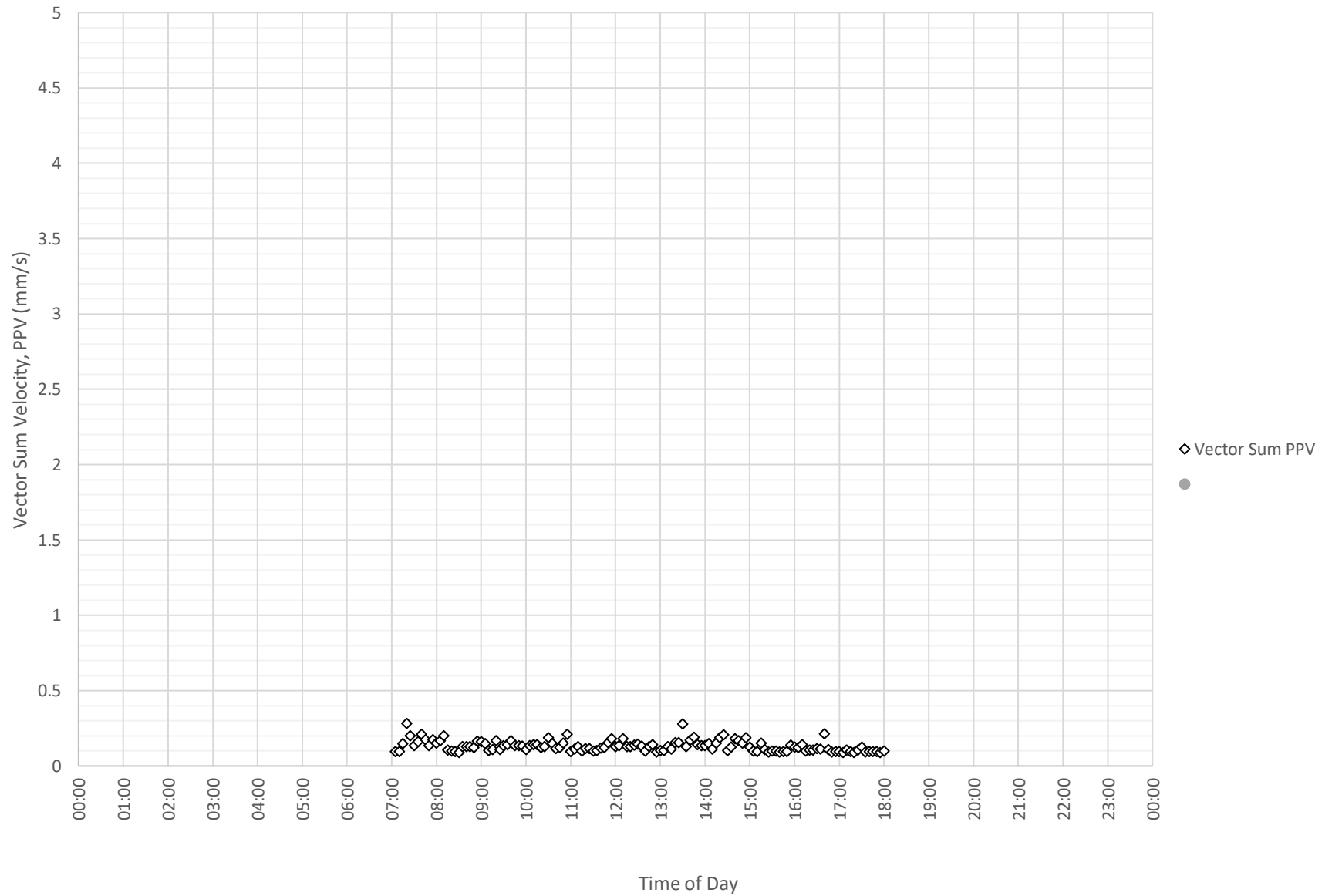
Daily Monitored Vibration Levels at Nepean Hospital Stage 2 - Level 2 Waiting Area (ETM7381) on 11-01-2024
