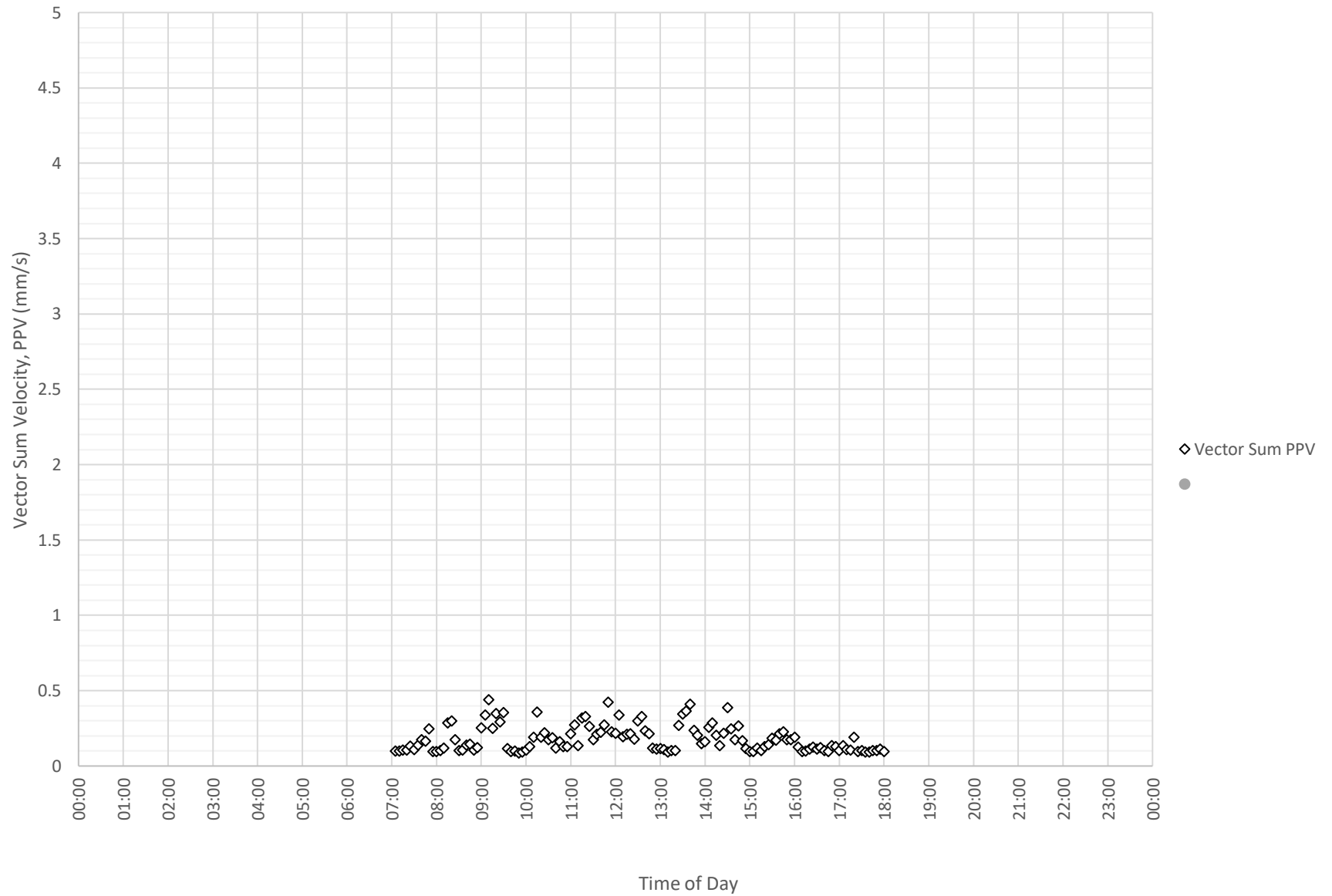
Daily Monitored Vibration Levels at Nepean Hospital Stage 2 - Level 2 Waiting Area (ETM7381) on 24-01-2024
