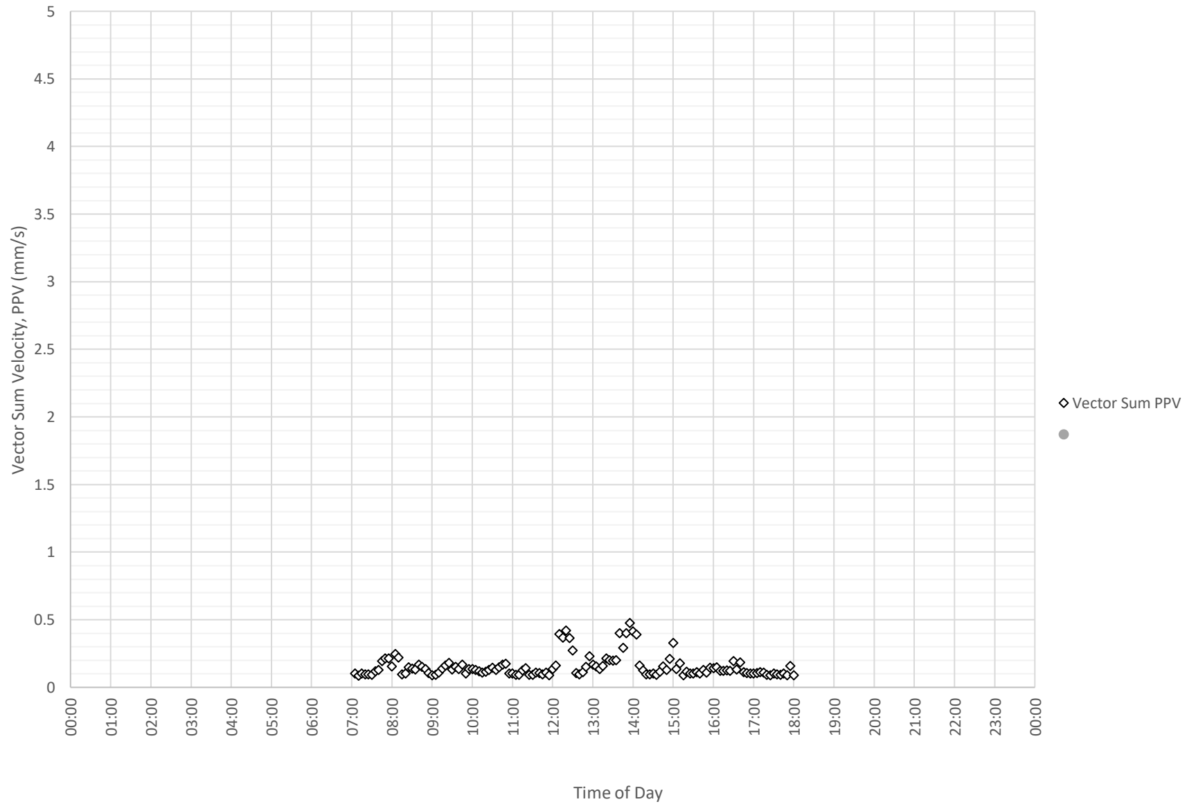
Daily Monitored Vibration Levels at Nepean Hospital Stage 2 - Level 2 Waiting Area (ETM7381) on 23-01-2024
