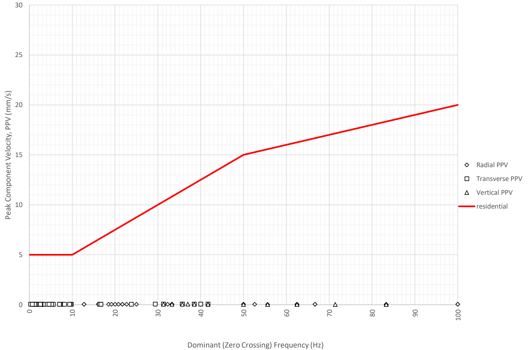
Frequency Content of Vibration Levels at Nepean Hospital Stage 2 - Tresillian Building (ETM7426) on 13-01-2024
