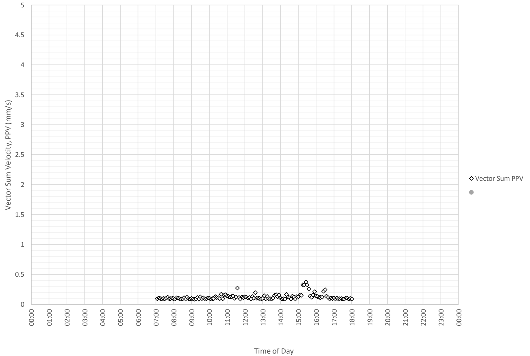
Daily Monitored Vibration Levels at Nepean Hospital Stage 2 - Level 2 Waiting Area (ETM7381) on 22-01-2024
