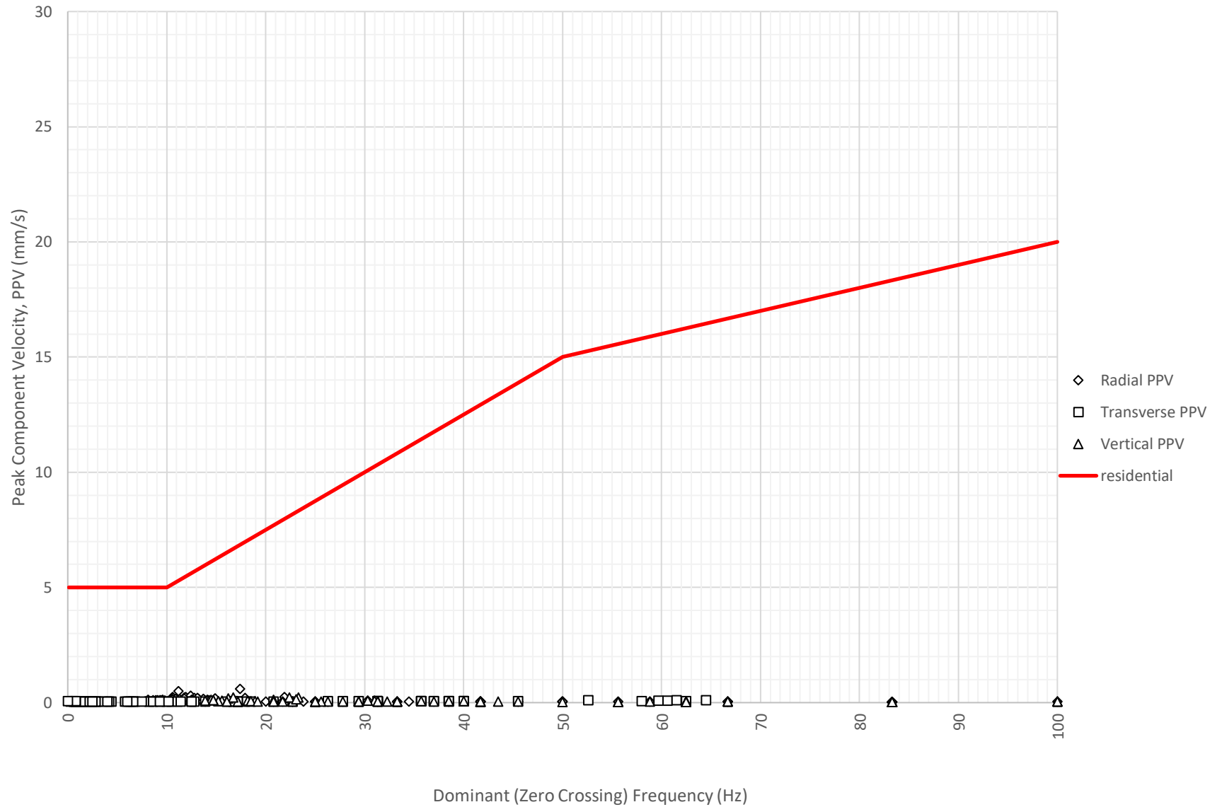
Frequency Content of Vibration Levels at Nepean Hospital Stage 2 - Tresillian Building (ETM7426) on 12-01-2024
