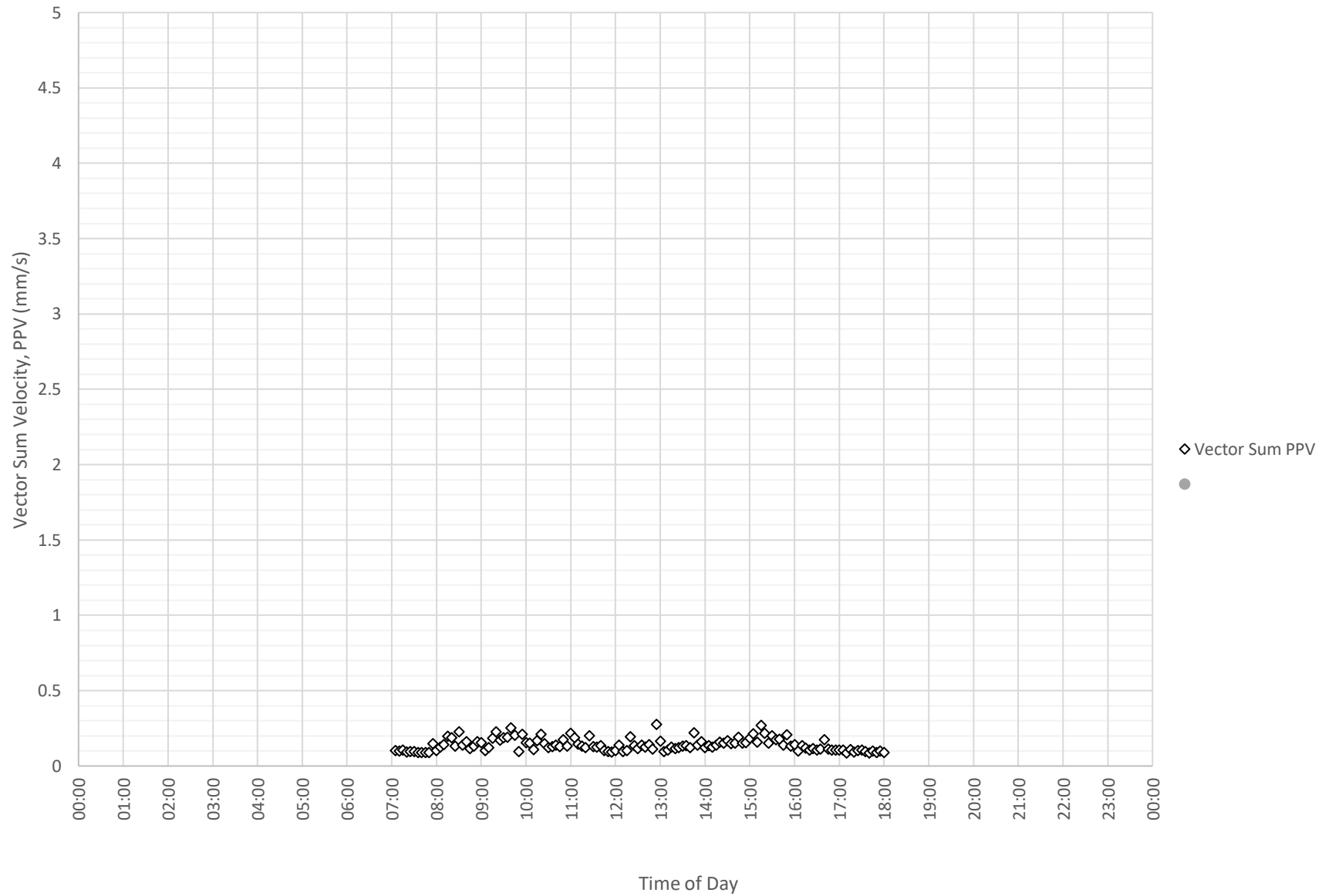
Daily Monitored Vibration Levels at Nepean Hospital Stage 2 - Level 2 Waiting Area (ETM7381) on 16-01-2024
