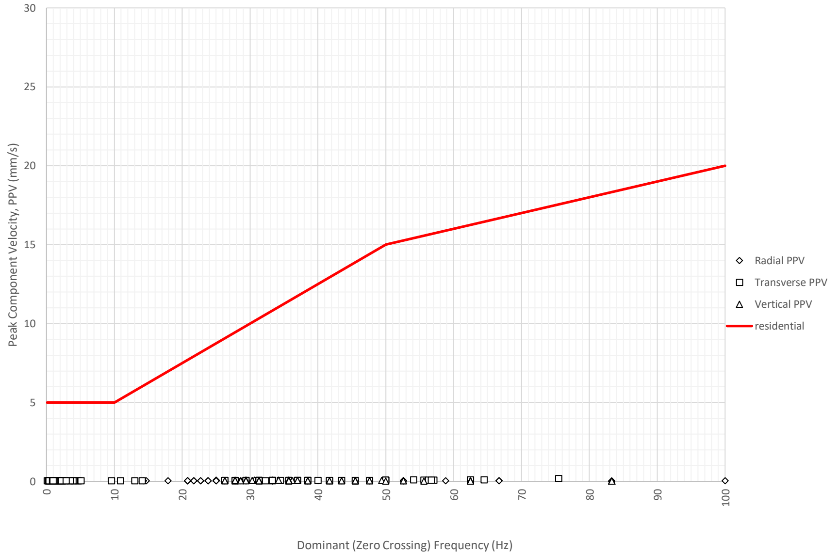
Frequency Content of Vibration Levels at Nepean Hospital Stage 2 - Tresillian Building (ETM7426) on 25-01-2024
