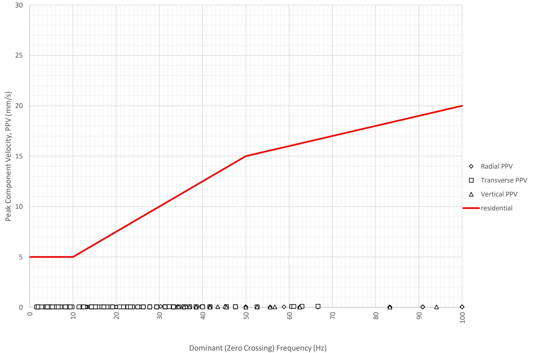
Frequency Content of Vibration Levels at Nepean Hospital Stage 2 - Tresillian Building (ETM7426) on 15-01-2024
