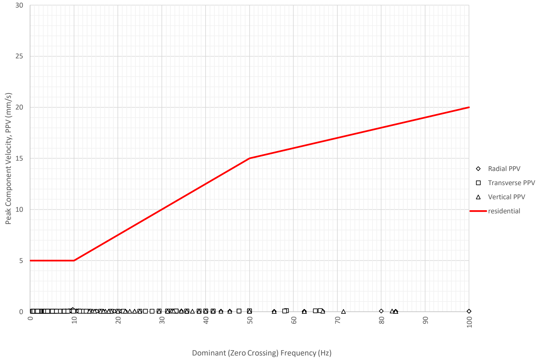
Frequency Content of Vibration Levels at Nepean Hospital Stage 2 - Tresillian Building (ETM7426) on 22-01-2024
