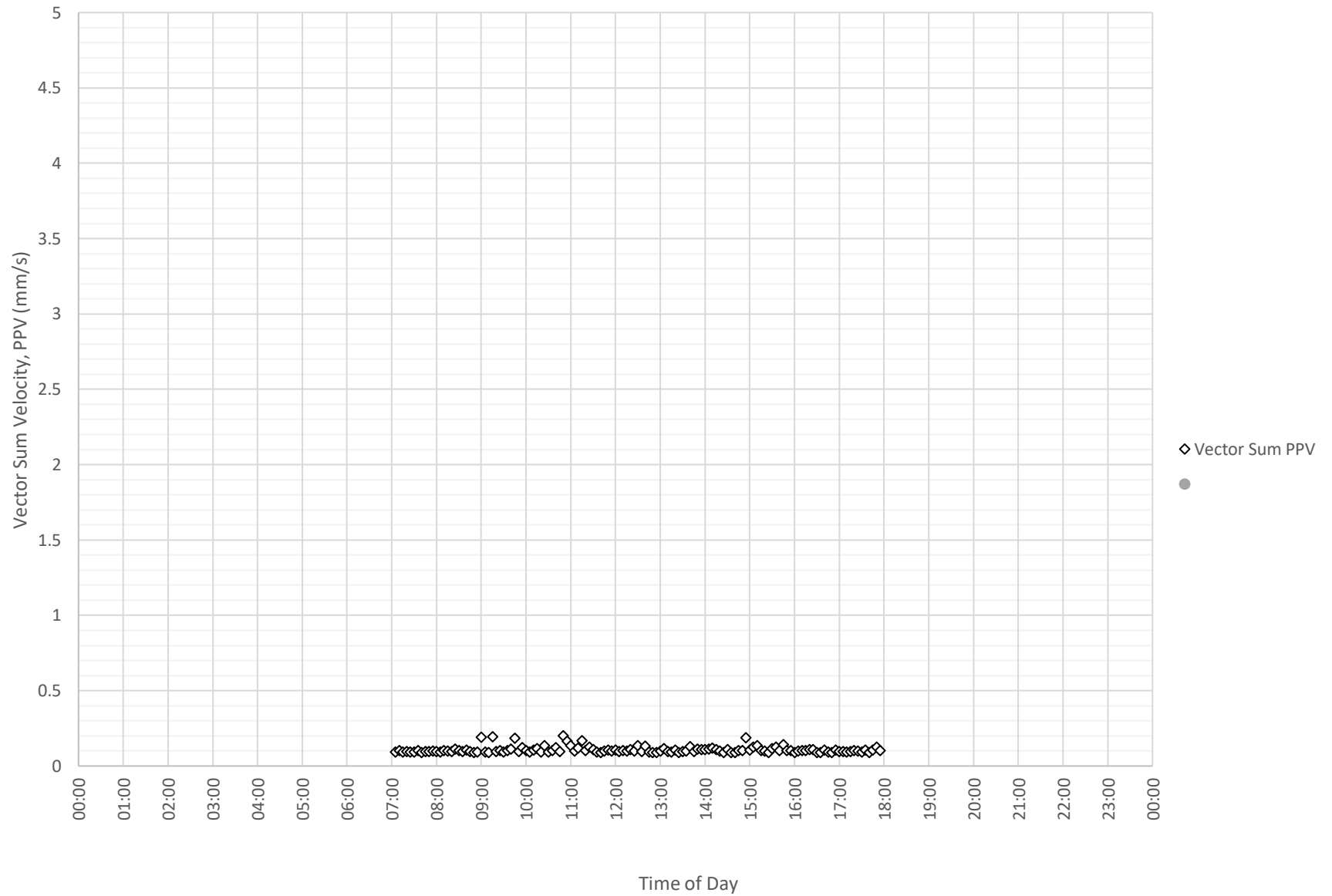
Daily Monitored Vibration Levels at Nepean Hospital Stage 2 - Level 2 Waiting Area (ETM7381) on 25-01-2024
