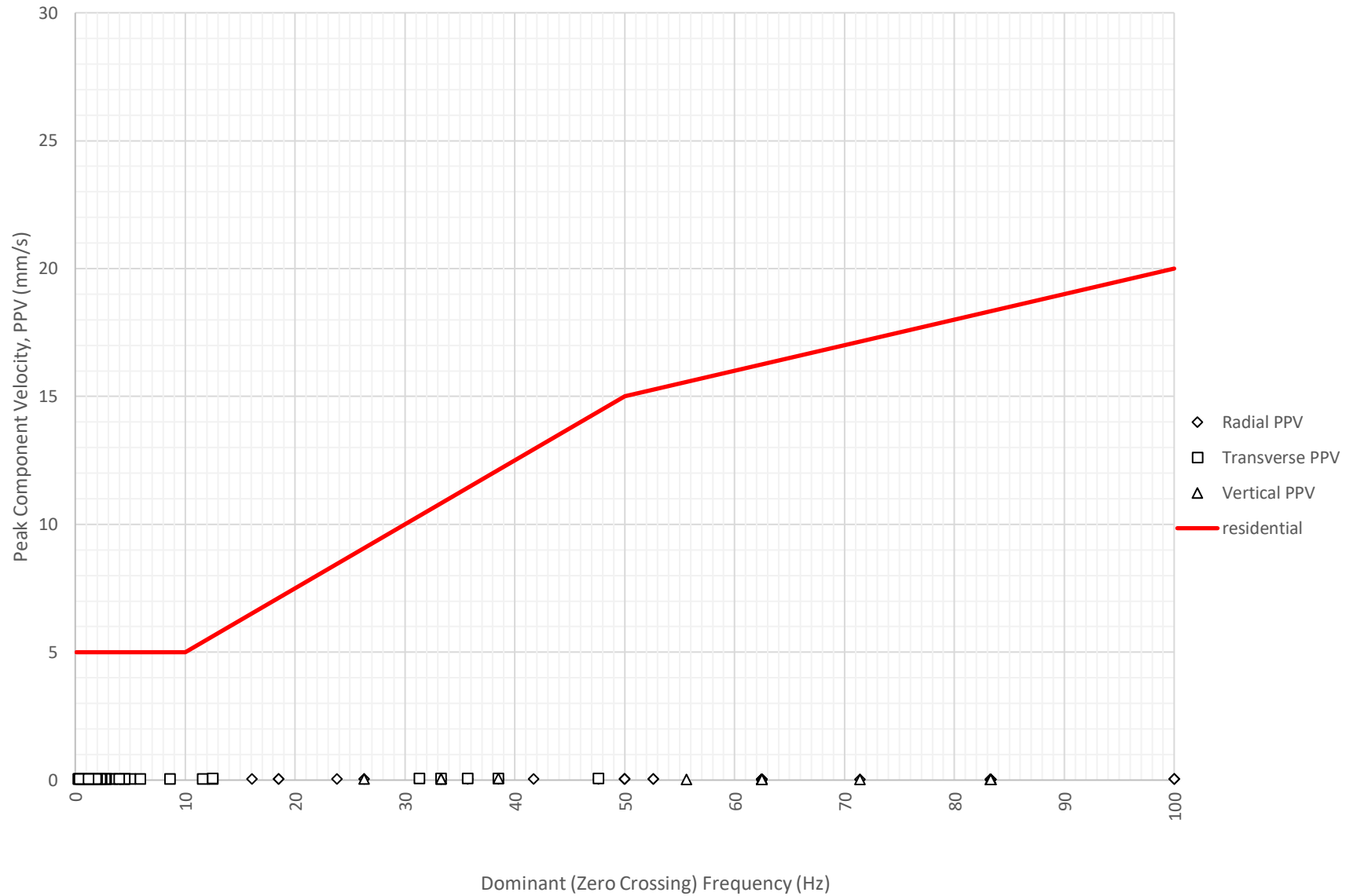
Frequency Content of Vibration Levels at Nepean Hospital Stage 2 - Tresillian Building (ETM7426) on 20-01-2024
