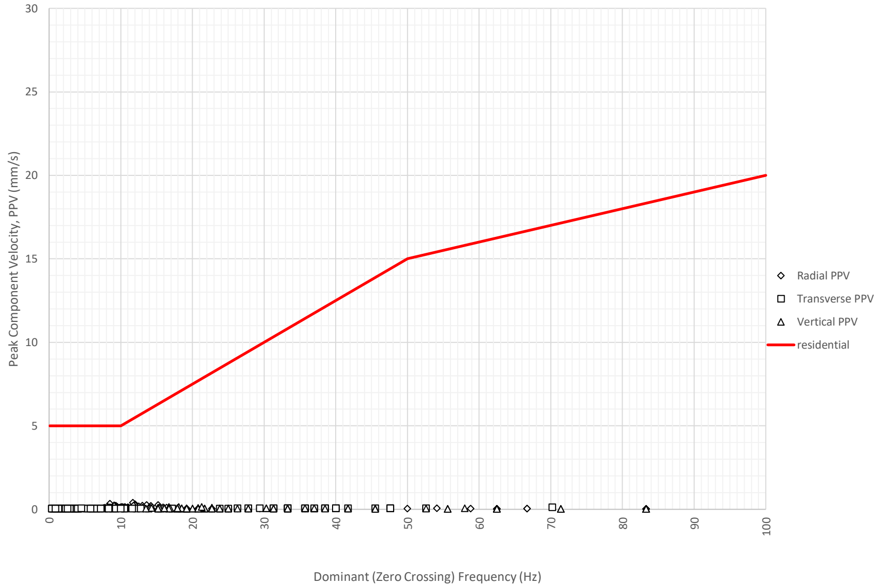
Frequency Content of Vibration Levels at Nepean Hospital Stage 2 - Tresillian Building (ETM7426) on 16-01-2024
