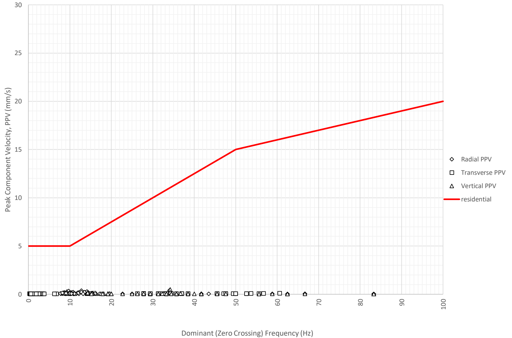
Frequency Content of Vibration Levels at Nepean Hospital Stage 2 - Tresillian Building (ETM7426) on 17-01-2024
