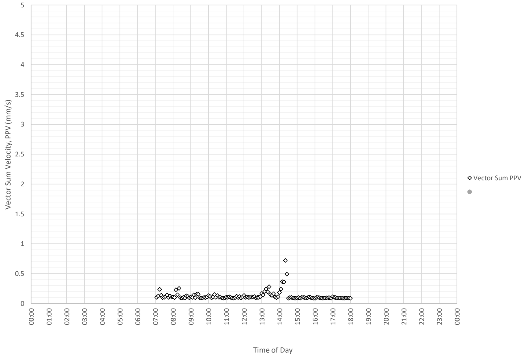
Daily Monitored Vibration Levels at Nepean Hospital Stage 2 - Level 2 Waiting Area (ETM7381) on 19-01-2024
