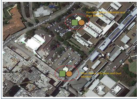
Figure 1: Noise, Vibration and Dust monitoring locations
